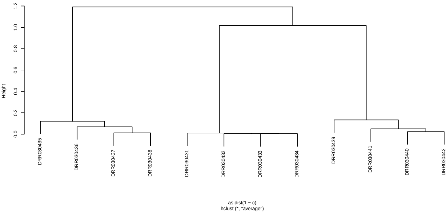
Cluster Dendrogram
